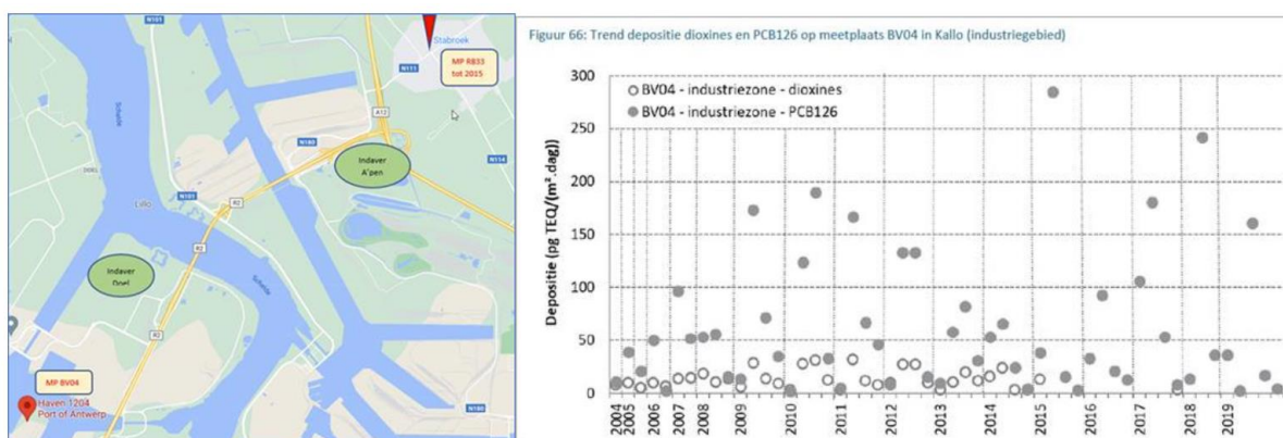
Figure 6: Monitoring of dioxin depositions around a Belgian WtE plant. On the left figure the two plants are indicated in green and the predicted deposition areas in red (MP BV04 and MP R833). The right figure shows the deposition of dioxins (pg TEQ/(m².dag)) from 2004 to 2019. Since 2015 the stations have no longer measured dioxin depositions (clear bullet points) due to the low values. MP R833 has completely disappeared, MP BV04 only measures PCB depositions (dark bullet points) due to scrap processing nearby. Source: Indaver, Belgium
