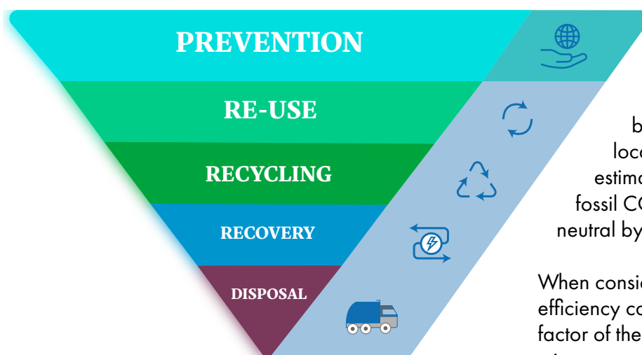
Figure 1: Waste Hierarchy
